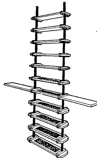
Pilot Ladder 11
