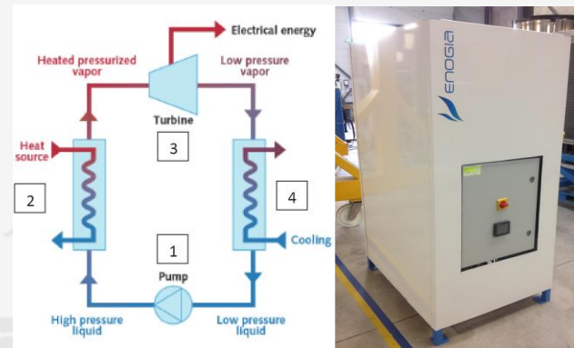
Organic Rankine Cycle: recover the waste heat generated on a Maritime Application
