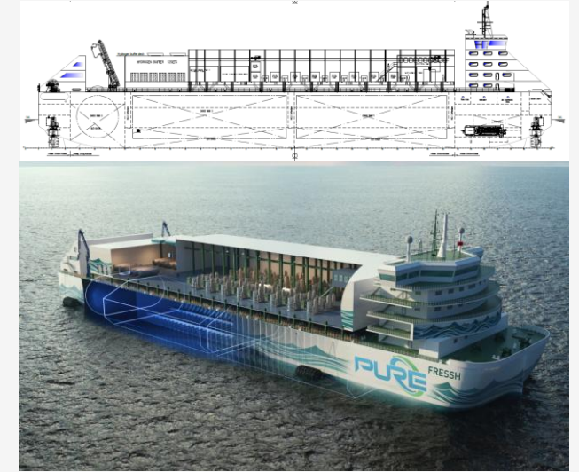
A seagoing Floating Renewable Energy Solution for Hydrogen vessel (FRESH) capable of storing and supplying hydrogen
