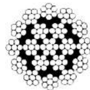
19X7
