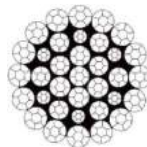
35X7+WA
