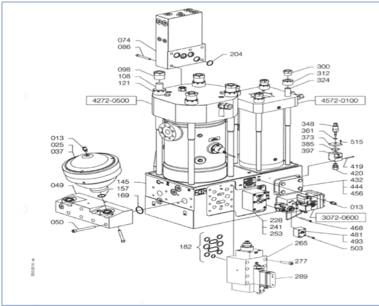
Complete Hydraulic Cyl. Unit
