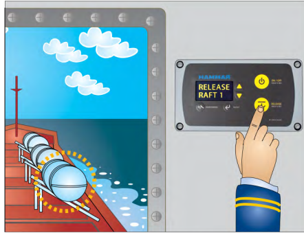
Electronic Remote Release System – ERRS.
