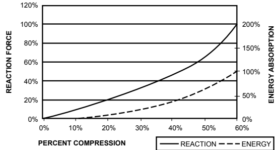
GENERIC PERFORMANCE CURVE OCEAN GUARD FENDER
