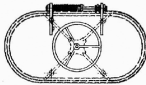
#215 SPRING BALANCED OVAL QUICK ACTING HATCH
