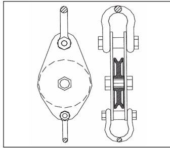
Single Sheave Block with Shackle
