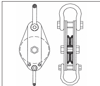
Single Sheave Block with Shackle
