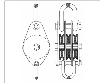
Triple Sheave Block with Shackle
