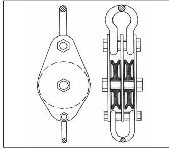
Double Sheave Block with Shackle
