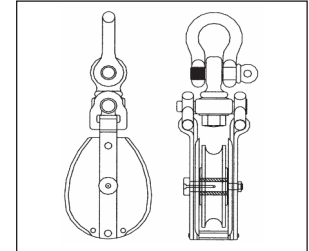
Steel Shell Block with Drilled Swivel Eye & Shackle
