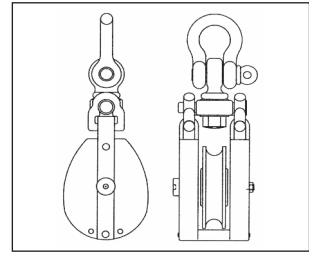
Wood Shell Block with Drilled Swivel Eye & Shackle
