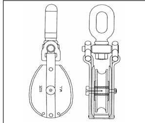
Steel Shell Block with Oblong Swivel Eye
