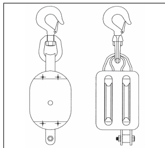
Double Sheave Block with Swivel Hook
