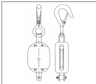
Single Sheave Block with Fixed Hook
