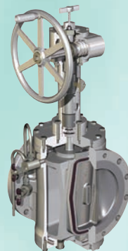
Cameron TwinSeal
