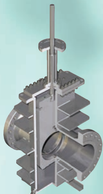
Cameron Grove skydeventil
