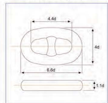
Enlarged link (E.L)
