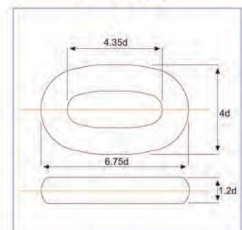
End link (E)
