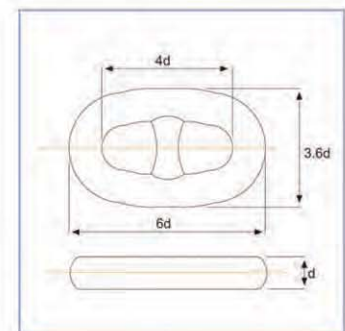
Common Link (C)
