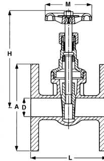
Fig. 291 – Gate Valve PN 16
