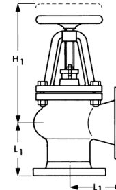
Fig. 1271 (short) Fig. 1271 DIN (long) Angle Valve
