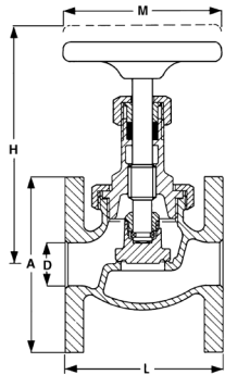
Fig. 275 – Globe Valve
