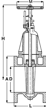
Fig. 1317 – Gate Valve
