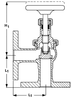
Fig. 276 – Angle Valve
