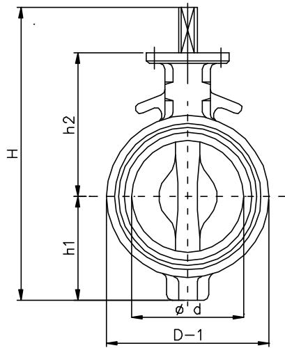
Wafer type.....Series 50
