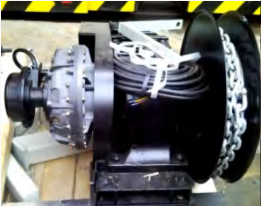
Rope Stabilizing Drum
