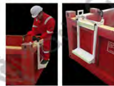
PORTABLE CONTAINER PLATFORM Portatif Konteyner Platformu
