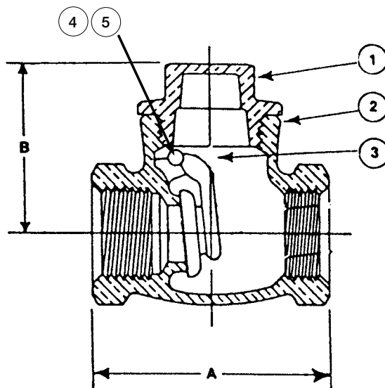
UP967 Threaded
