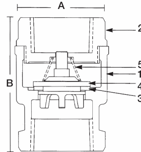
Check Valve Figure #548T 250 lb. WOG In-Line Spring Loaded Check TFE Disc / Threaded Ends
