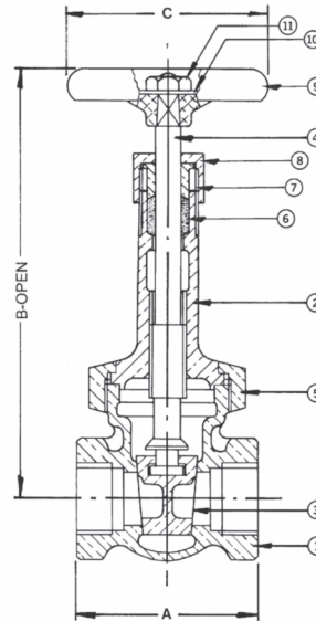
Figure #1182 300 lb. SWP-1000 lb. WOG • Rising Stem Union Bonnet • Cu/Ni Seat Rings • Threaded Ends
