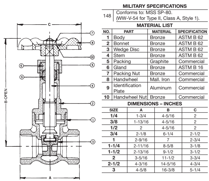
Figure #148 125 lb. SWP-200 lb. WOG • Rising Stem Threaded Bonnet • Threaded Ends
