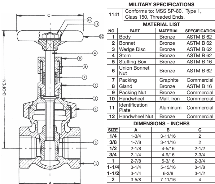
Figure #1141 150 lb. SWP-300 lb. WOG • Non-Rising Stem Union Bonnet • Threaded Ends
