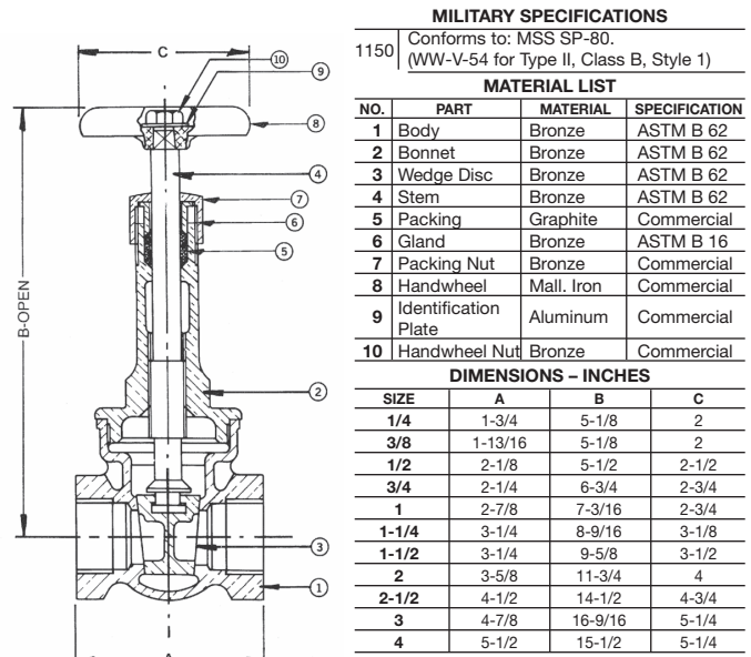
Figure #1150 150 lb. SWP-300 lb. WOG • Rising Stem Union Bonnet • Threaded Ends
