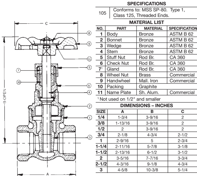
Figure #105 125 lb. SWP-200 lb. WOG • Non-Rising Stem Threaded Bonnet • Threaded Ends
