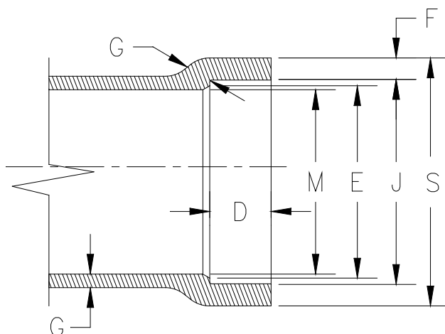
Socket Detail
