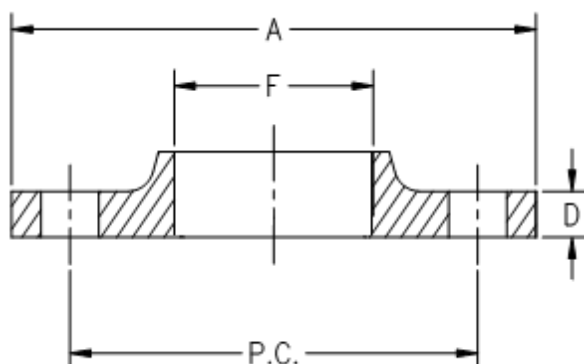
250 PSI Slip-On
