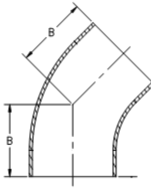
45° Elbows
