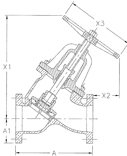
Flanged Globe Y Pattern Valve – Type 6
