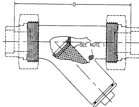
Union End Y-Strainer
