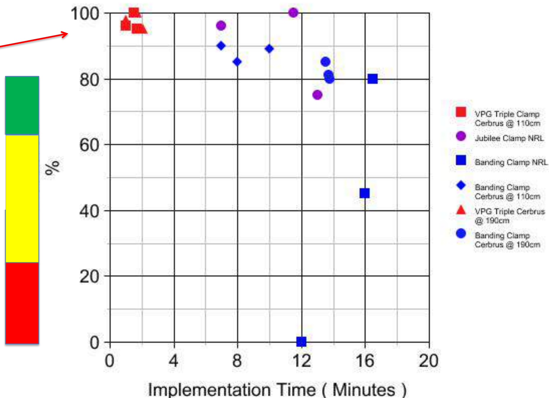
Performance comparison VPG Clamp vs Jubilee Clamp vs Banding Clamp
