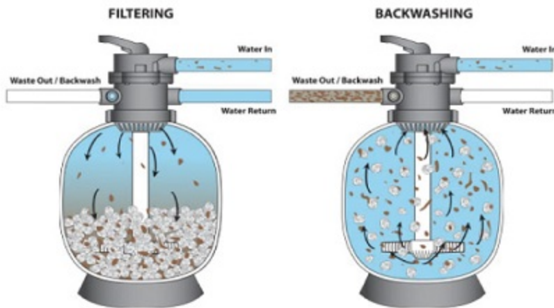
BACKWASH FILTER PROCESS
