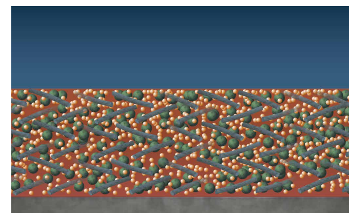
Fresh antifouling coating before exposure to seawater. The Smartfibres run parallel to the surface.
