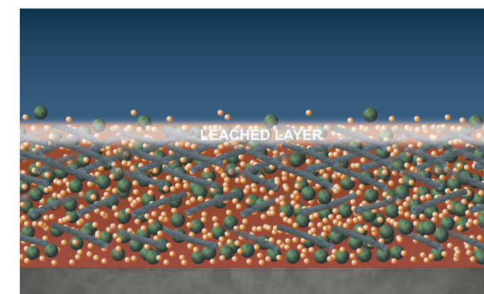
The antifouling coating after exposure to seawater. As a result of the biocide release, a leached layer starts to form. Water flow and the parallel structure of the fibres facilitates the smooth and uniform removal of the leached layer, ensuring a well-controlled polishing rate throughout the coating's entire service life.
